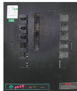
Strand Environ® rack with JSI JS-ENVY digital DMX 512 control
